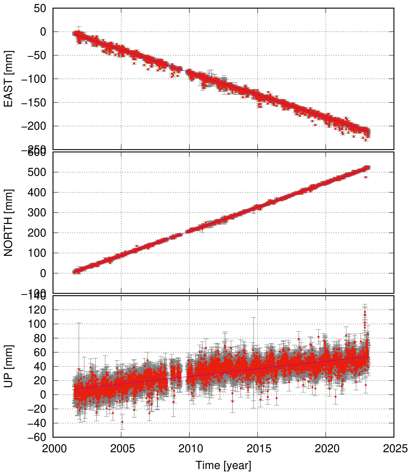
AKUR (65.69, -18.12) time series (ITRF 2014) v_e = -9.57 \pm 0.14 ; v_n = 23.89 \pm 0.12 ; v_u = 2.14 \pm 0.41 mm/yr
