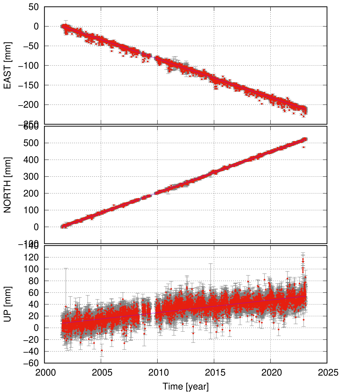
AKUR (65.69, -18.12) time series (ITRF 2014) v_e = -9.84 \pm 0.14 ; v_n = 24.23 \pm 0.14 ; v_u = 2.14 \pm 0.41 mm/yr
