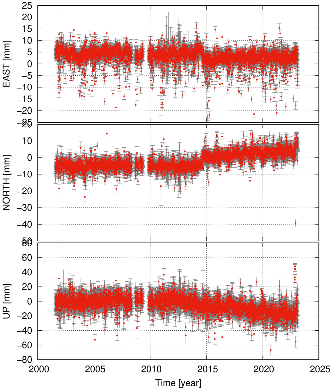
AKUR detrended and seasonal signal removed
