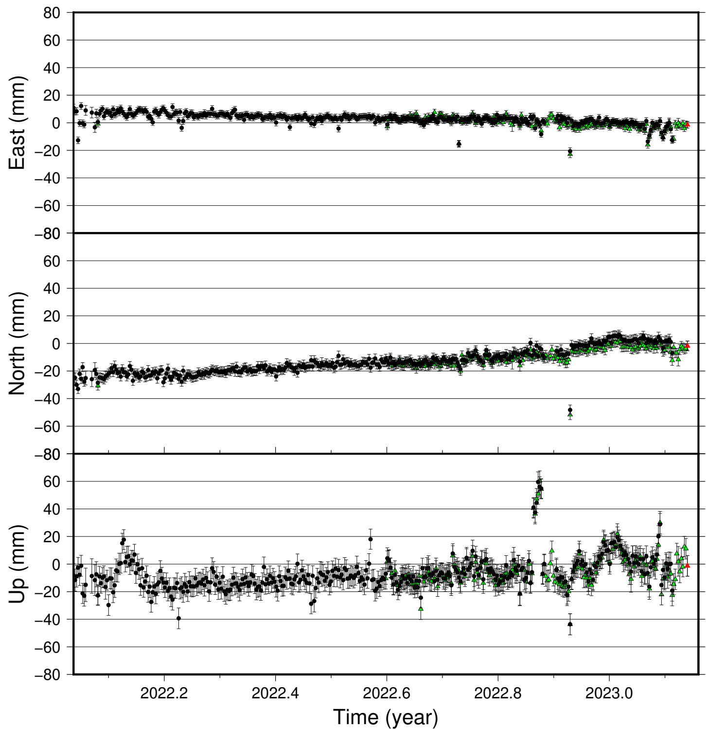
AKUR time series (IGS 2014), last 400 days
