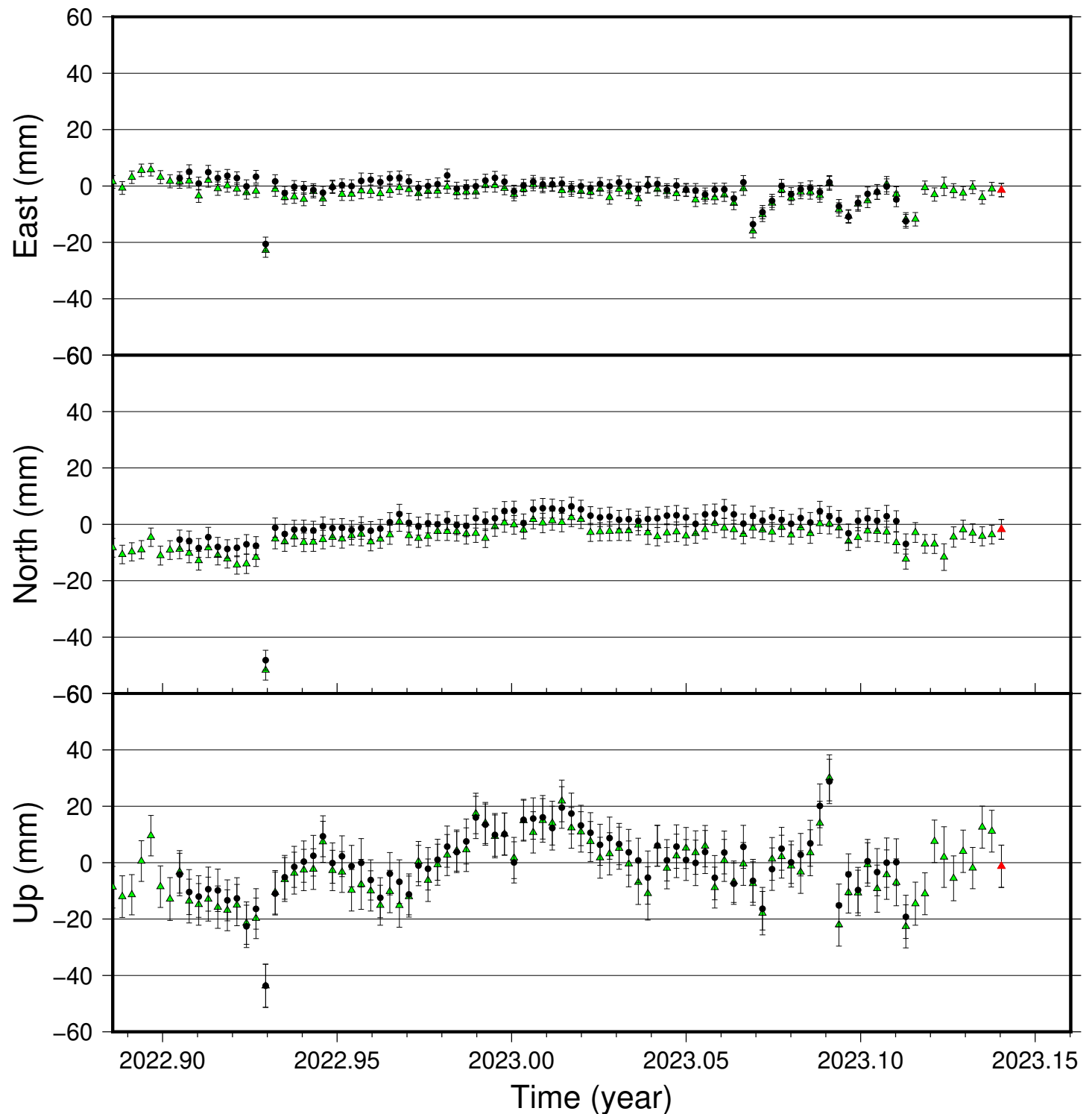
AKUR time series (IGS 2014), last 100 days
