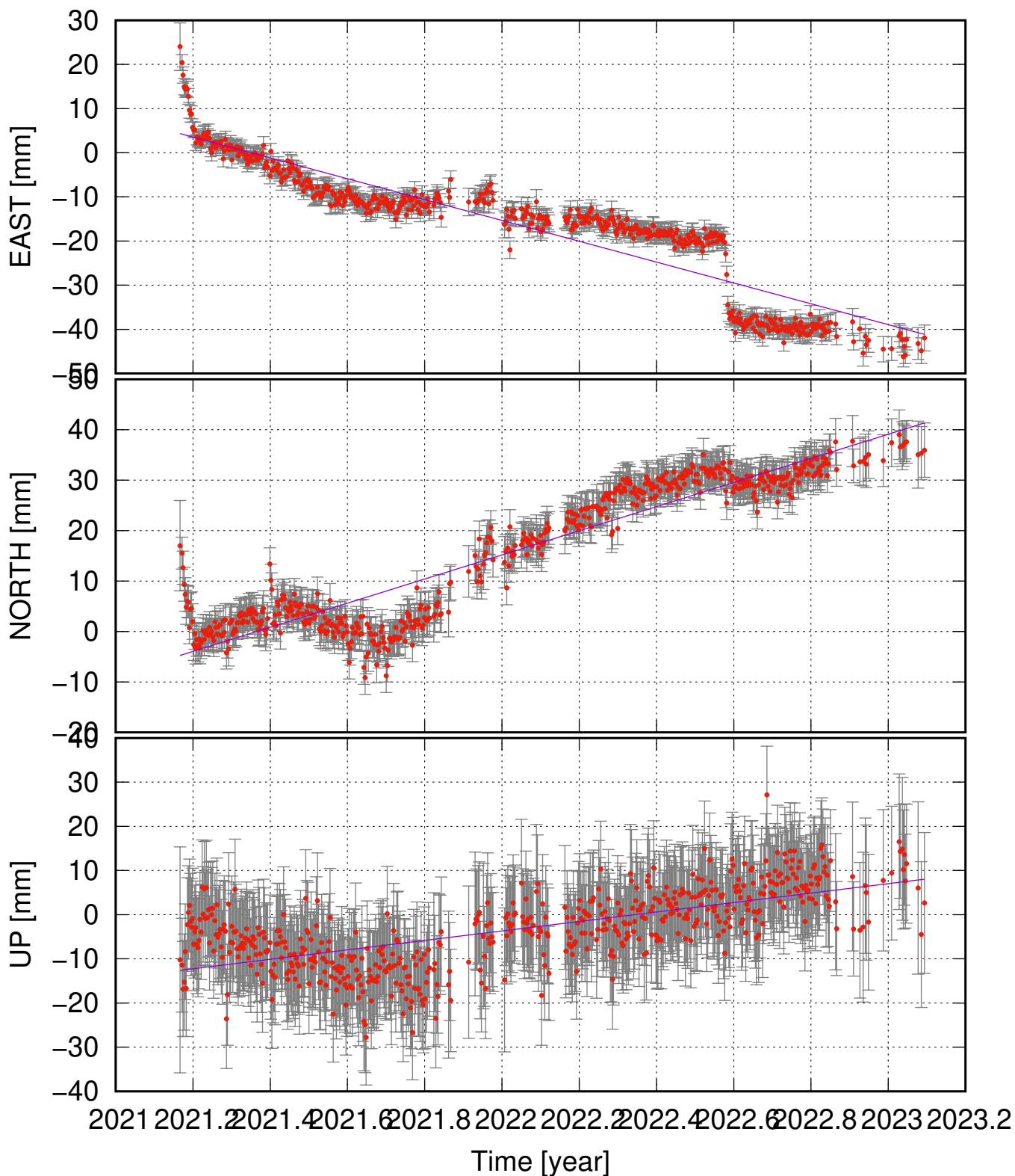
AFST (63.98, -22.14) time series (ITRF 2014) v_e = -23.60 \pm 2.80 ; v_n = 23.92 \pm 2.59 ; v_u = 10.70 \pm 3.33 mm/yr
